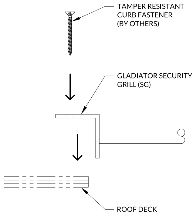
POSITION GLADIATOR SECURITY GRILL OVER ROOF OPENING
